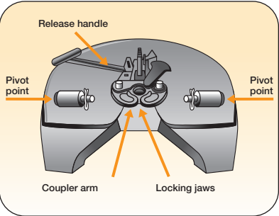
Parts of a fifth wheel.
